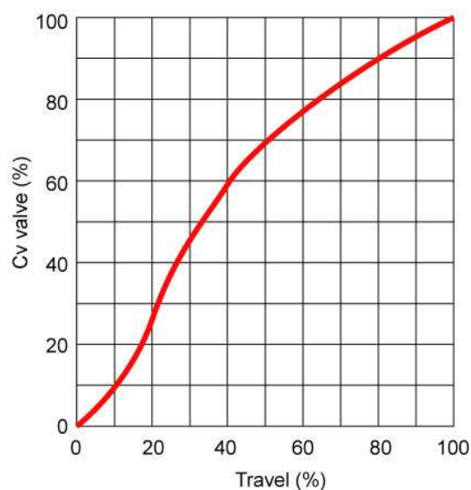
Fig. 1-1-2 linear characteristics (Ltf : soft seat)
