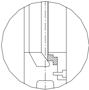
Teflon Seat
