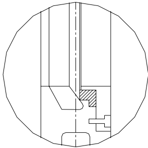
Rubber Seat
