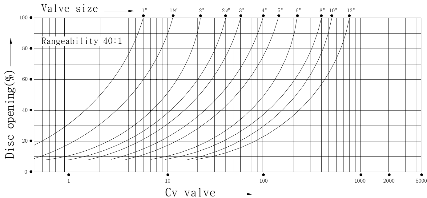
Fig. 5-3 40% Reduced Bore Flow Characteristics Valve size →
